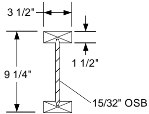
END DETAIL TYP.
