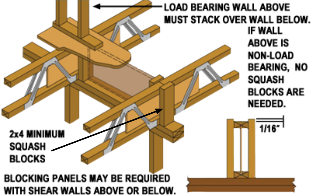
DETAIL B — INTERIOR BEARING WITH SQUASH BLOCKS
