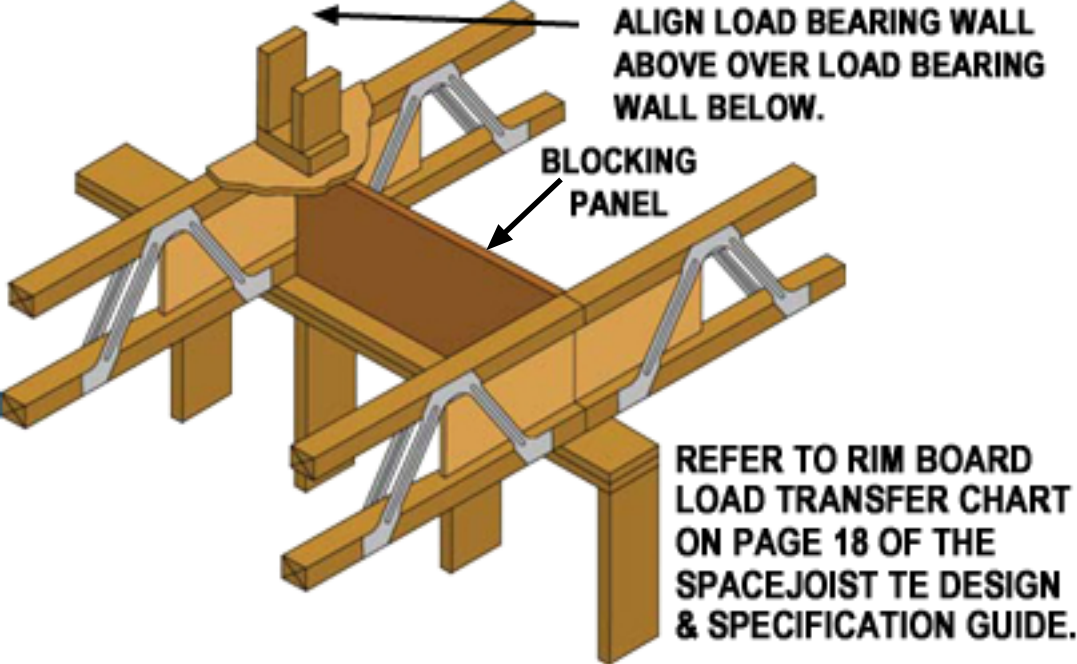
DETAIL C — INTERIOR BEARING WITH BLOCKING PANEL
